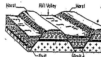
Fig. 2.11 Rift Valley
