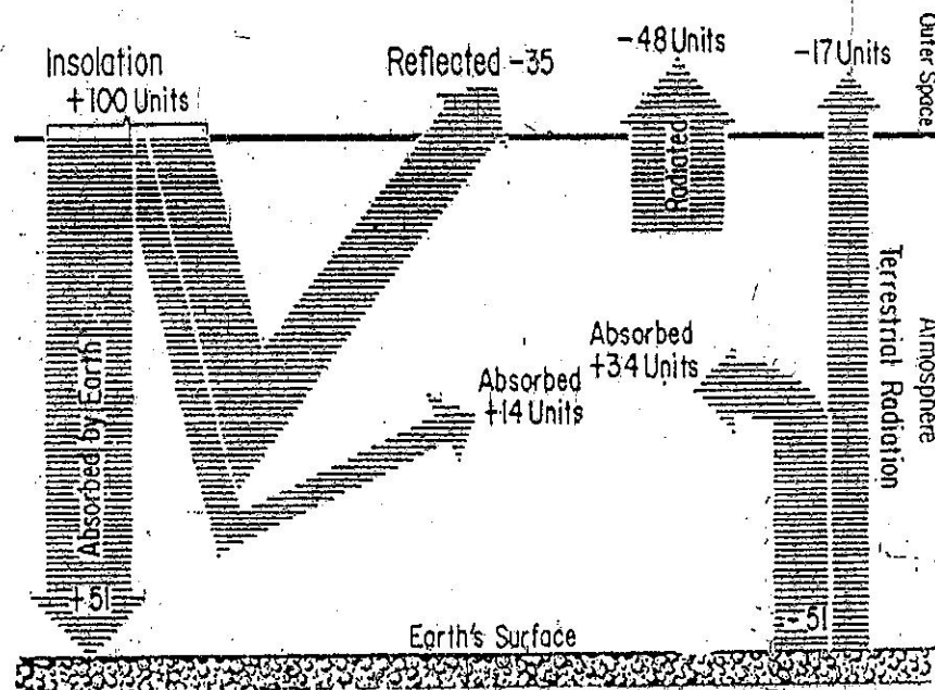
Fig. 4.1 Insolation Heat balance of the Atmosphere.
