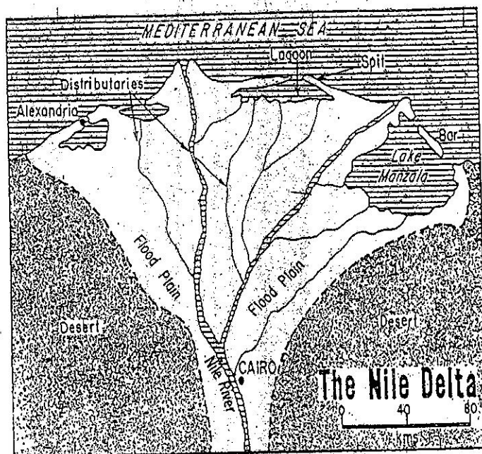
Fig. 2.5 A Delta
