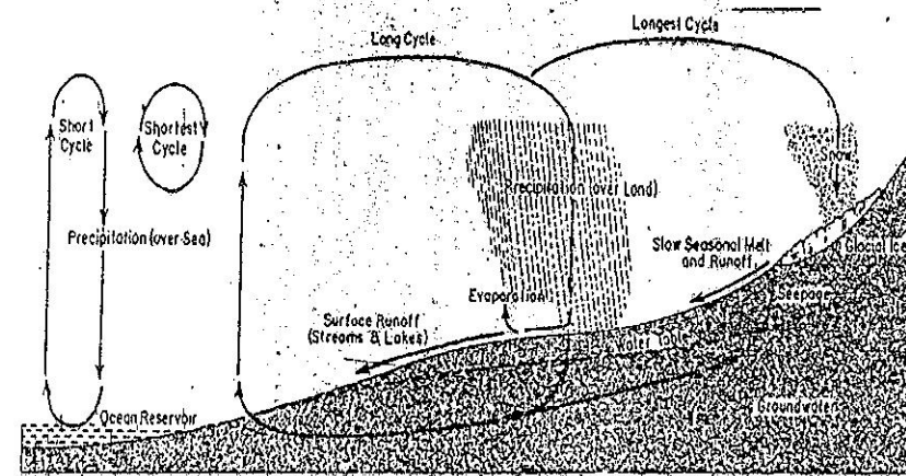
Fig. 3.4 Hydrological Cycle
