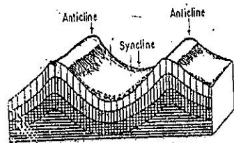
Fig. 2.12 Simple Folds
