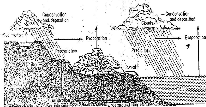
Fig. 1.5 Hydrological Cycle
