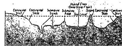
Fig. 3.1 Submarine Relief
