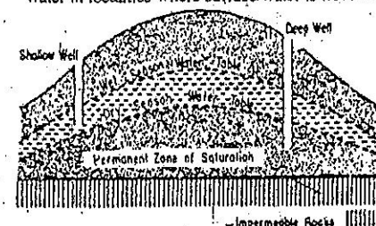
Fig. 3.3 (a) Water Table
