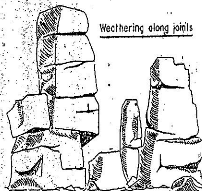
Fig. 2.1 (a) Weathering of Rocks. Water enters the rocks through their joints. In course of time they are split up.
