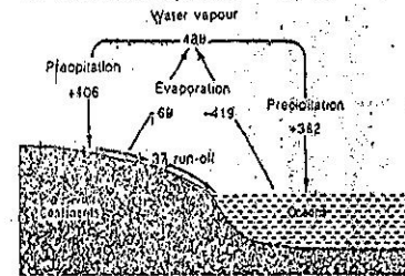
Fig. 3.5 Water Balance
