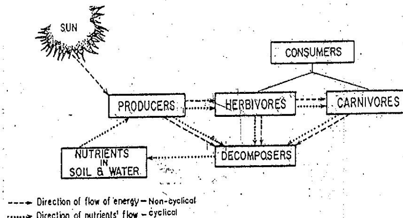
Fig. 3.2 Cycle of Energy and Nutrients Flow in Ecosystem
