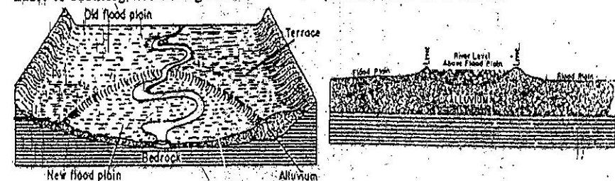
Fig. 2.4 (a) Meanders
