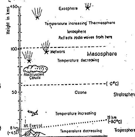
Fig. 1.2 Structure of the Atmosphere
