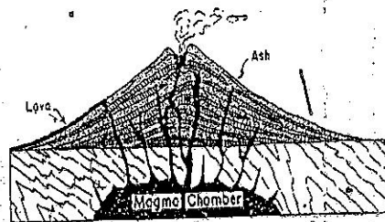
Fig. 2.13 Volcanic Cone with a Crater
