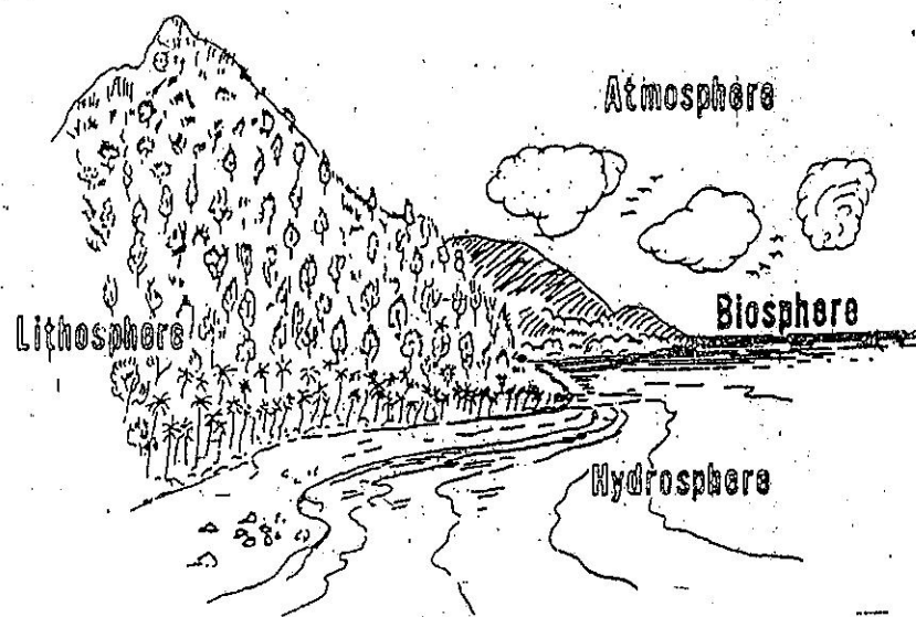
Fig. 1.6 The Biosphere
