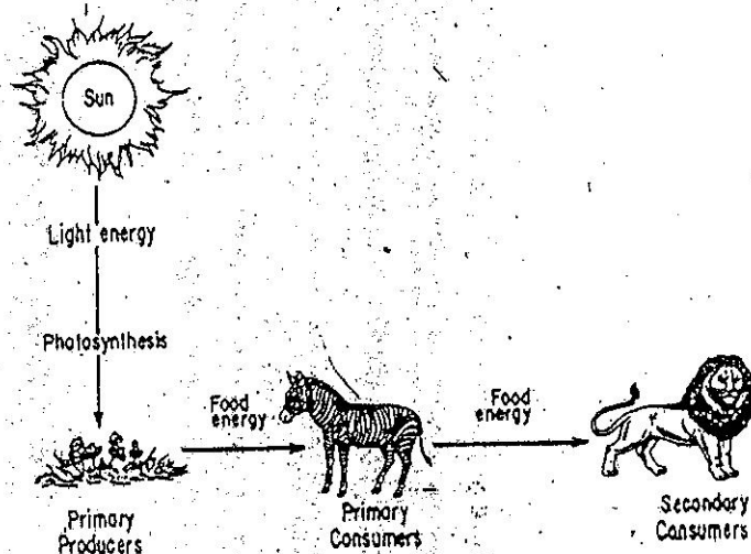
Fig. 3.1 Food Chain
