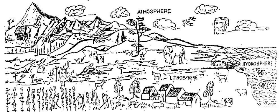
Fig. 18 The biosphere
