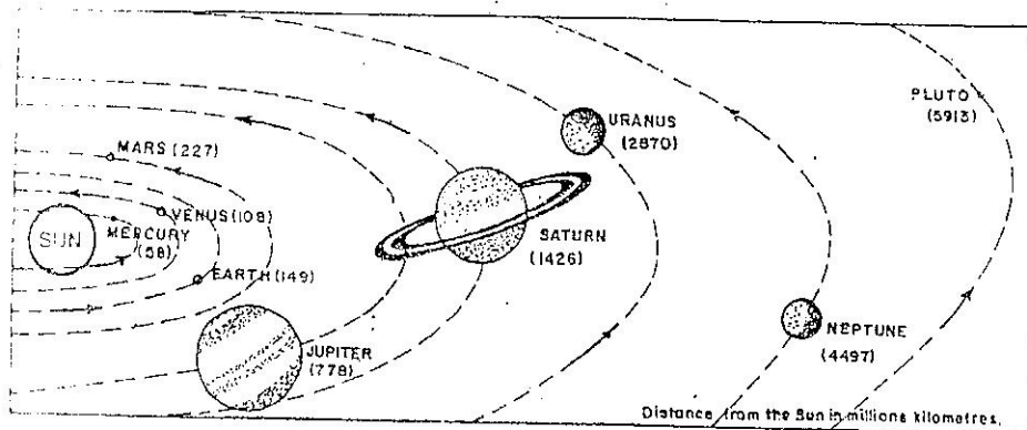
Fig. 1-The solar system
