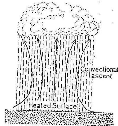
Fig. 3.3 Convective rainfall The warm, moist air rising upwards forms clouds and gives rise to sudden and heavy showers called convective rainfall.
