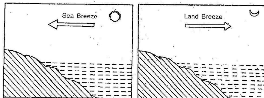
Fig. 2.5 Sea breeze and land breeze
