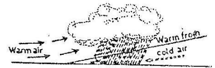
Fig. 3.4 Cyclonic rainfall The uplifting of the warm air in a cyclone causes this rainfall.
