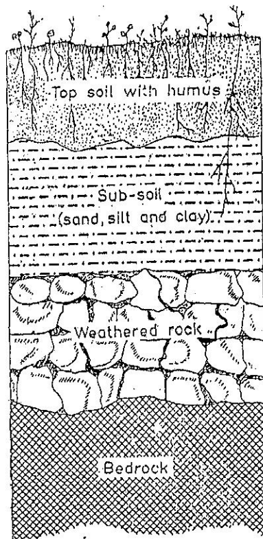
Fig. 3 Formation of soil
